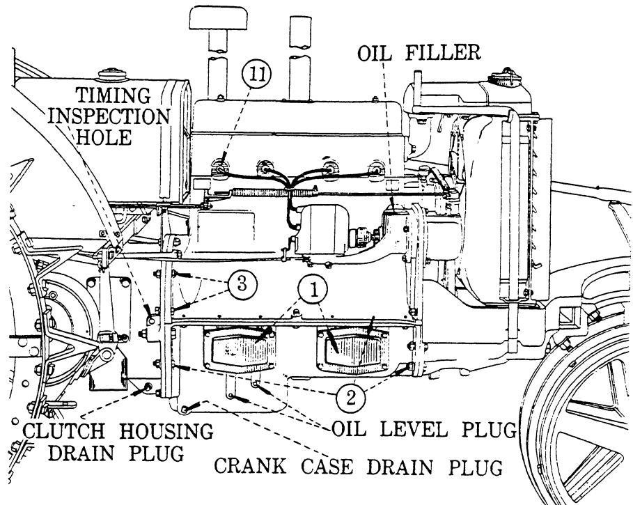
Fig. 4. R. H. Side of Case "CC" Tractor
