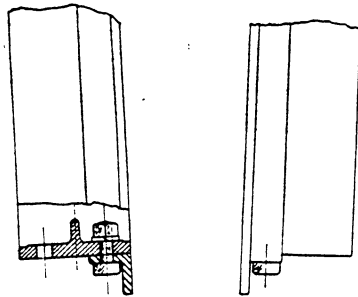
No. 2. Position of Front Wheel Skid Rings for Flat Ground Operation.
