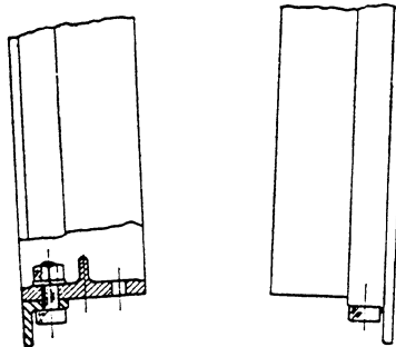
Fig. 3. Position of Front Wheel Skid Rings for Riding Listed Ridges.
