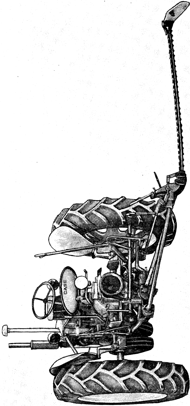
Figure 1. Mower on Model "DC" Tractor Equipped with a Hydraulic Lift
