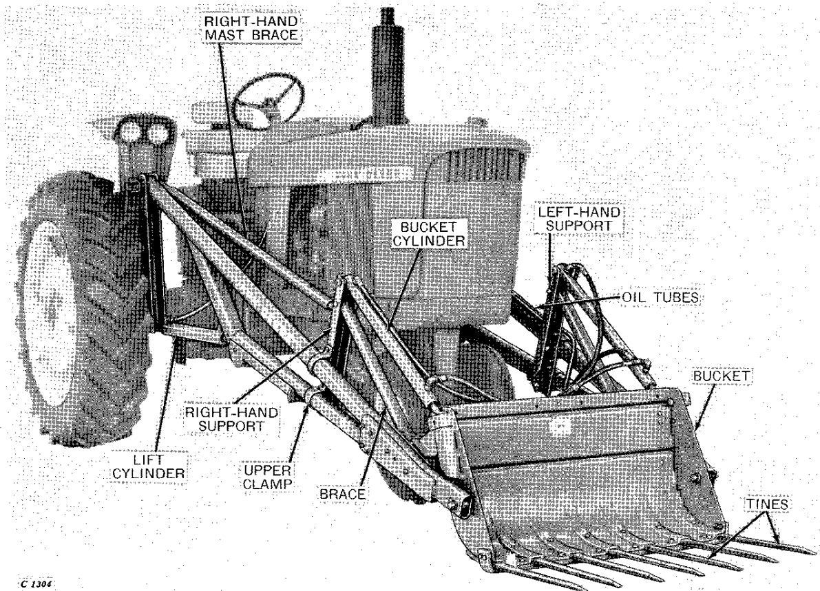
John Deere 45 Farm Loader with Hydraulically-Controlled Bucket on John Deere 3010 Tractor
