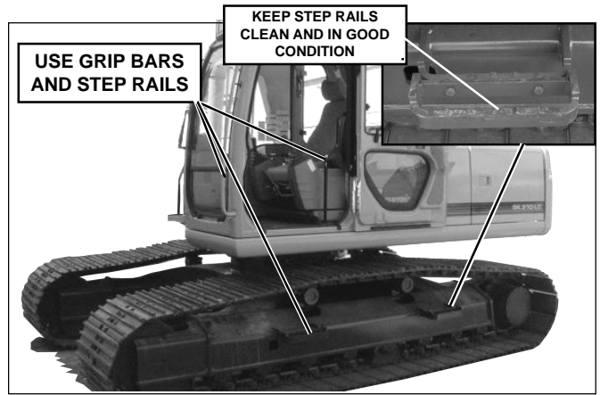
MOUNTING/DISMOUNTING MACHINE
